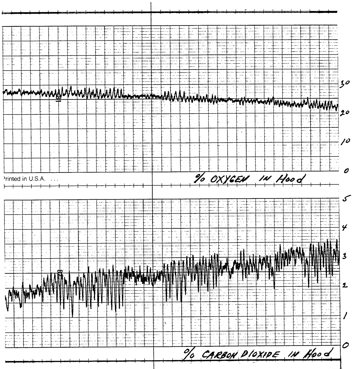
Figure 9 - Air Supply System Manned Test Results.
