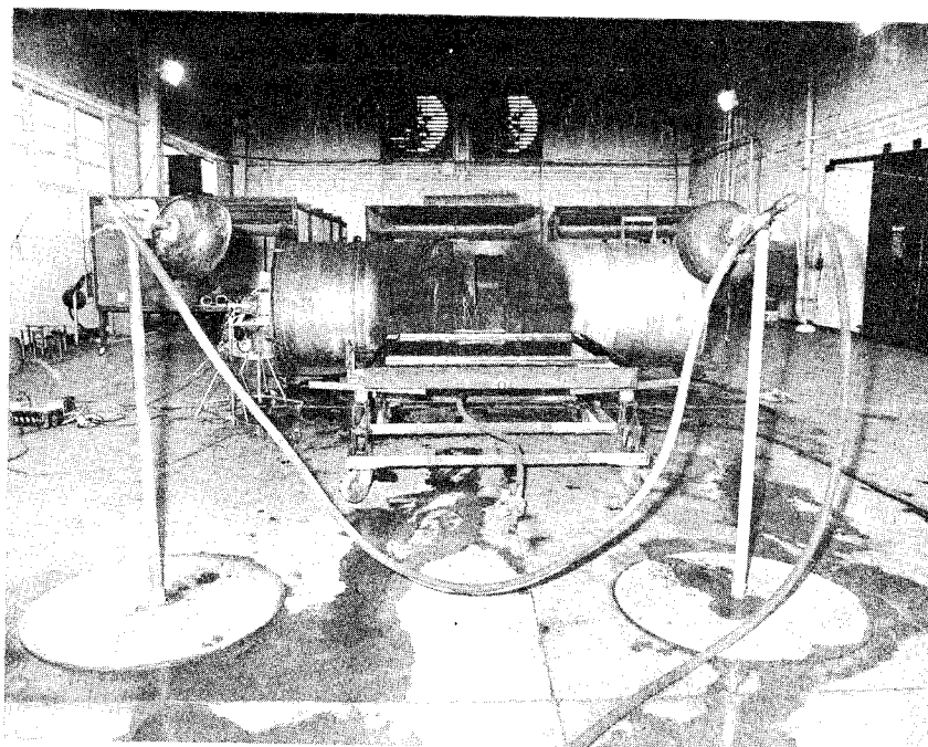
a. OVERALL VIEW OF TEST BED
