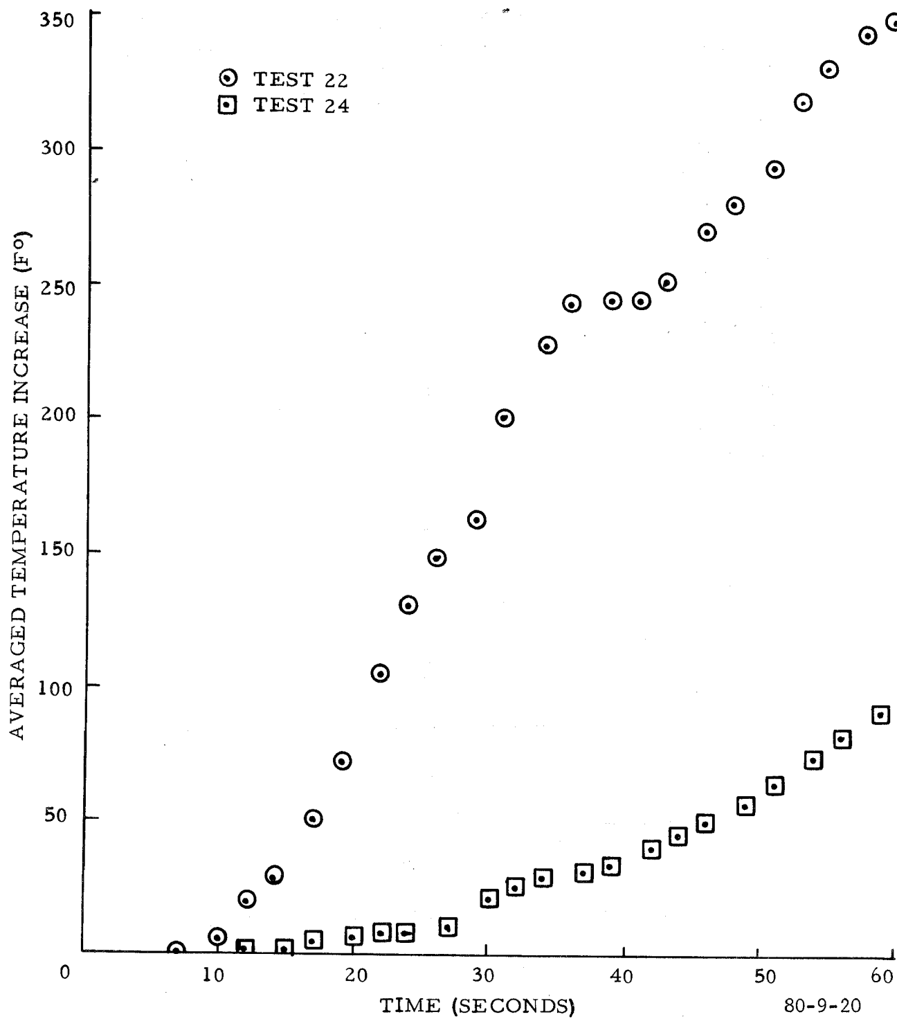
FIGURE 20. TEMPERATURE INCREASE (TESTS 22 AND 24)
