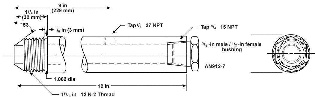
Figure E1-8. Btu Heat Transfer Device—Outlet Tube
