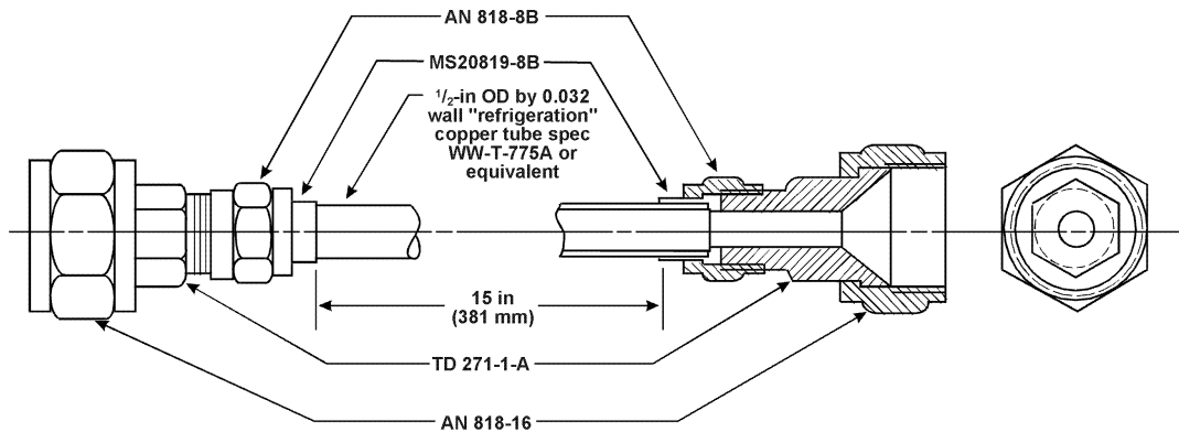
Figure E1-10. Btu Heat Transfer Device—Test Specimen
