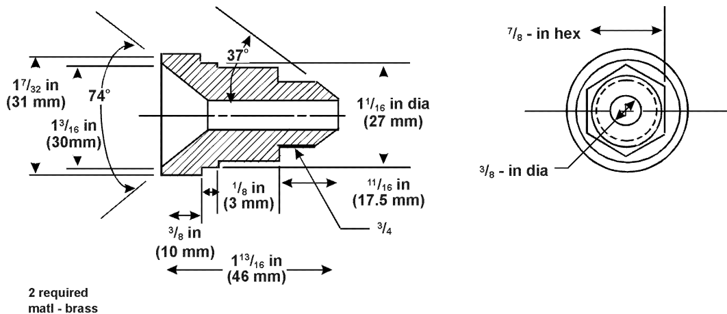
Figure E1-6. Btu Heat Transfer Device—Reducer
