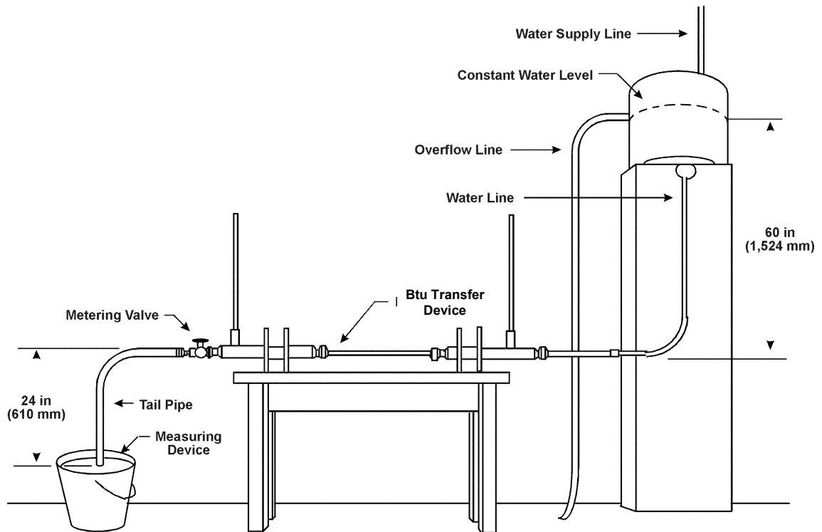
Figure E1-4. Burner Calibration Standardization Apparatus
