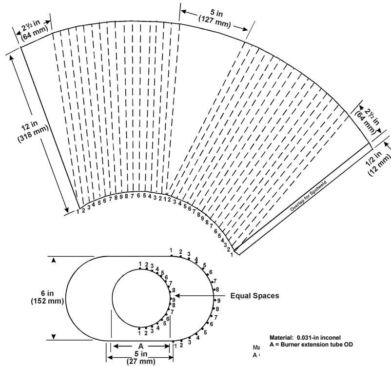
Figure E1-1. Burner Extension Funnel
