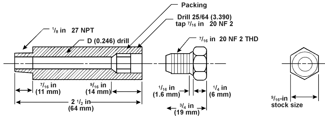
Figure E1-9. Btu Heat Transfer Device—Thermometer Mounting
