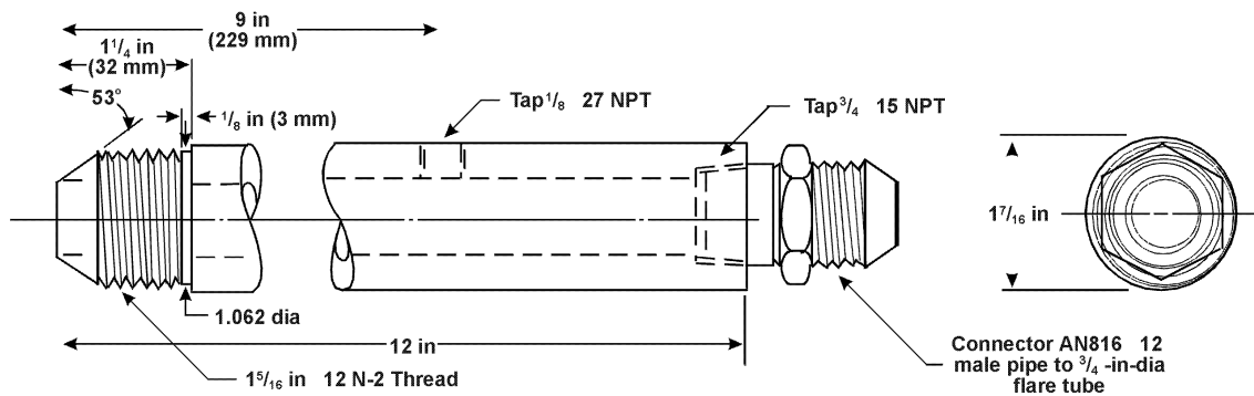
Figure E1-7. Btu Heat Transfer Device—Inlet Tube
