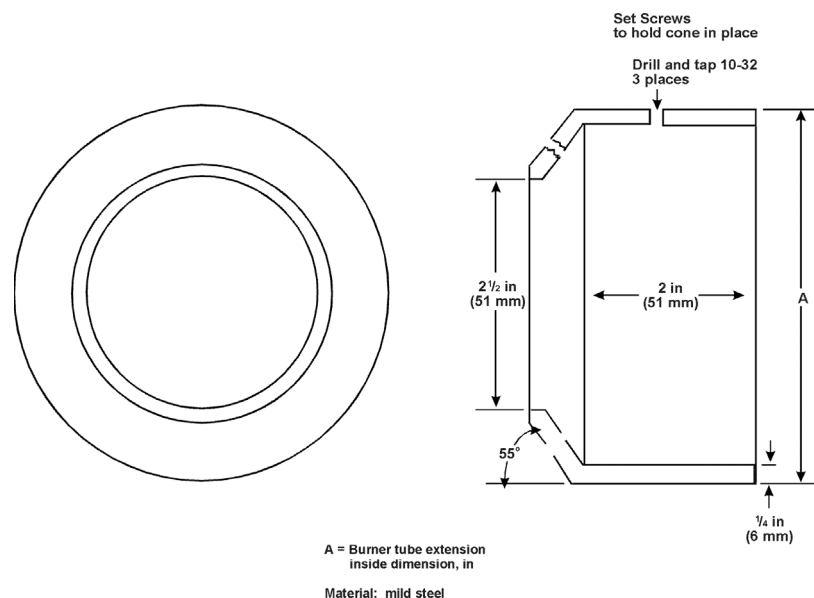
Figure E1-2. Air Tube Reducing Cone
