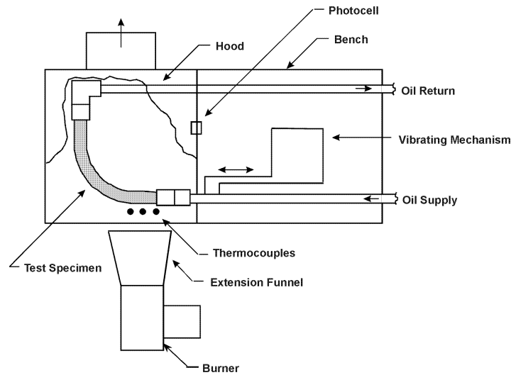
Figure E1-3. Hose Assemblies Test Setup
