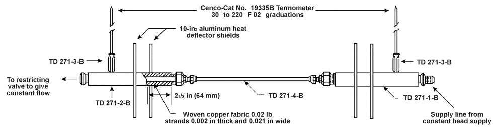
Figure E1-5. Btu Heat Transfer Device
