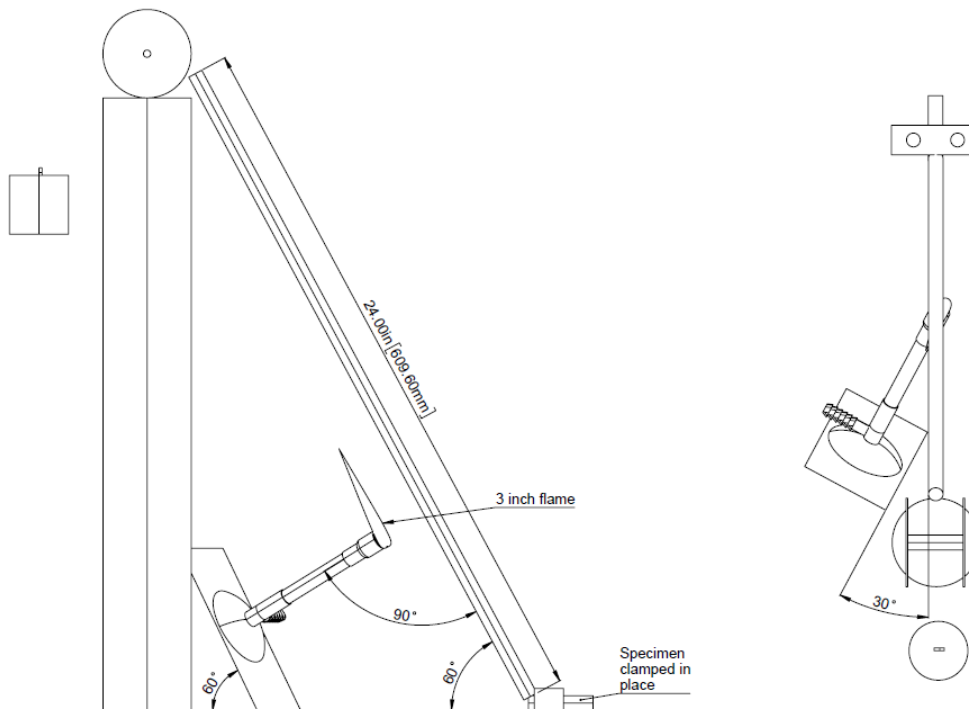
Figure 4-3. Alternative setup for 60-degree electrical wire Bunsen burner test
