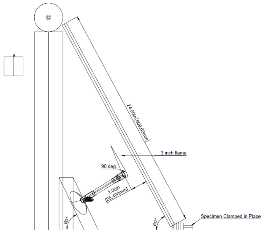
Figure 4-1. 60-degree electrical wire Bunsen burner test setup
