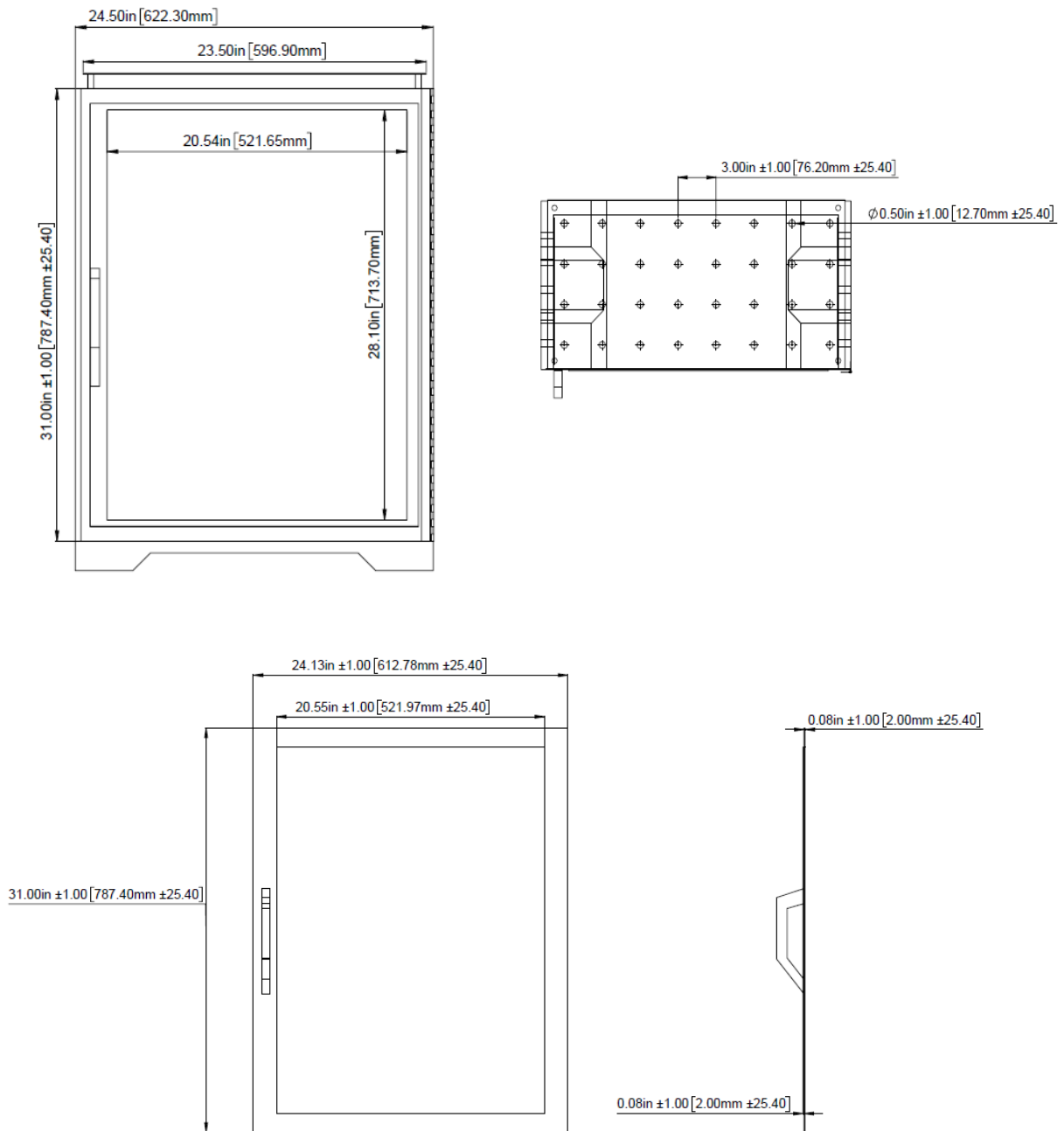
Figure 3-2. Front and top view of horizontal Bunsen burner test cabinet
