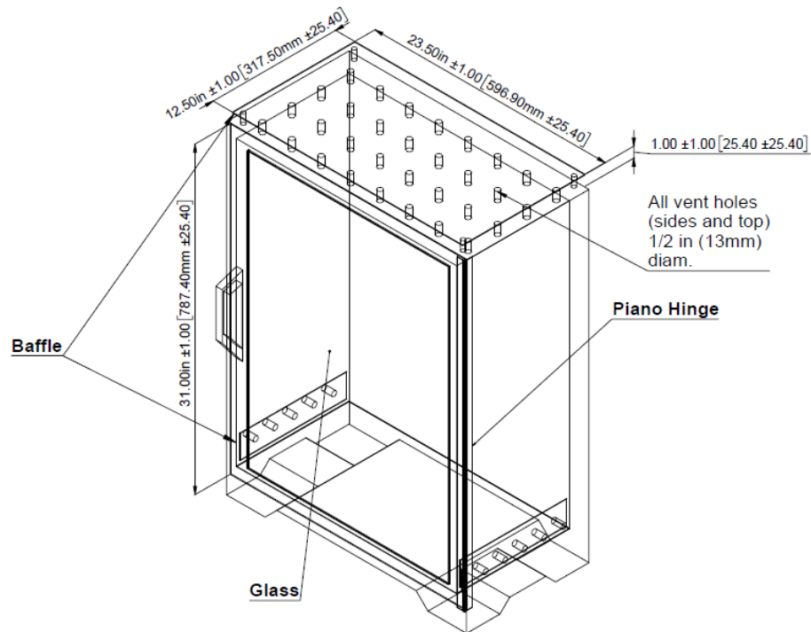
Figure 3-1. Sketch of horizontal Bunsen burner test cabinet
