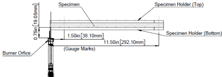
Figure 3-6. Typical burner and sample location
