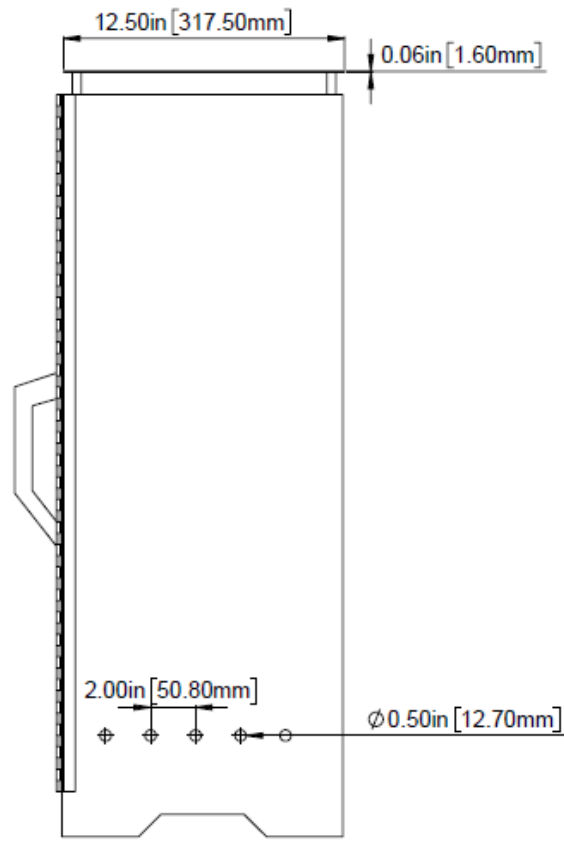
Figure 3-3. Side view of horizontal Bunsen burner test cabinet
