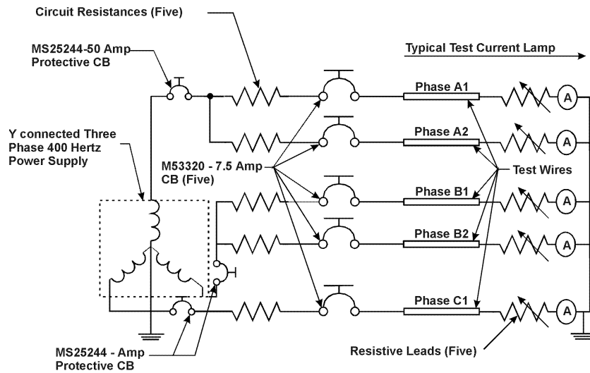
Figure 21-5. Electrical Connection
