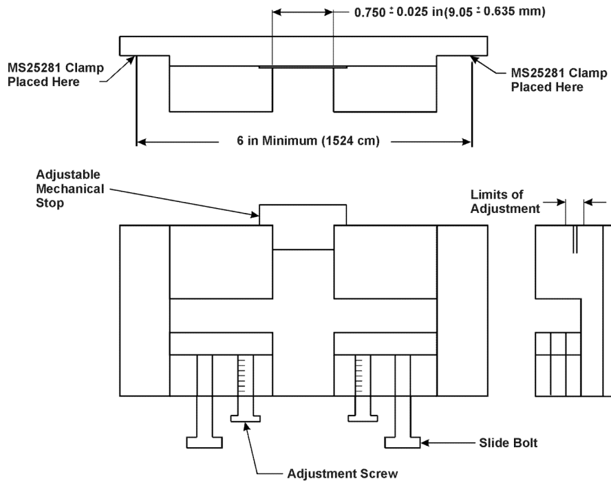
Figure 21-4. Test Fixture
