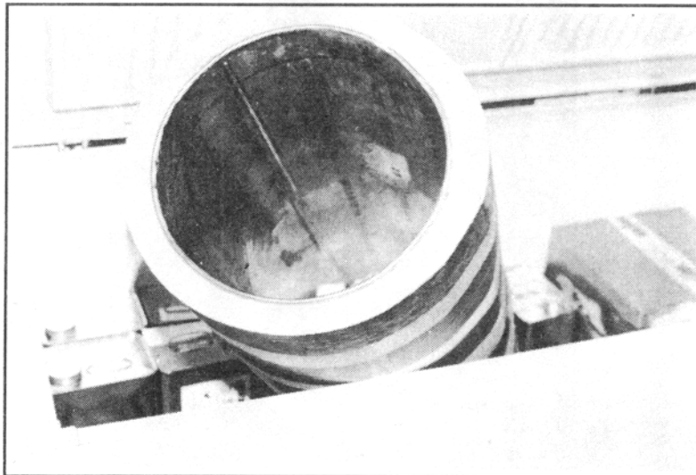
FIGURE B-2 347 Stainless Steel Insulated Enclosing Cylinder from Freezer for Dry Ice and Alcohol Bath
