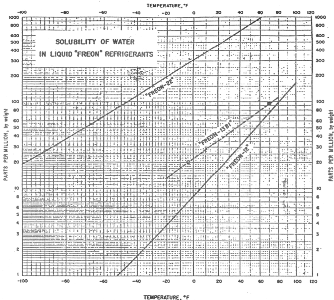
Solubility of Water in Liquid "Freon" Refrigerants.
