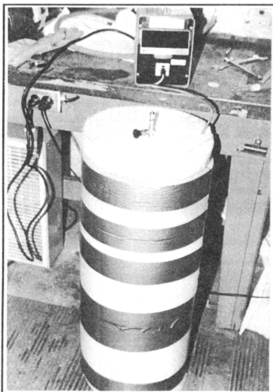
FIGURE B-13 About 30 Minutes Following Initial Dry Ice Introduction SCUBA Tank is at -80 Degrees Centigrade
