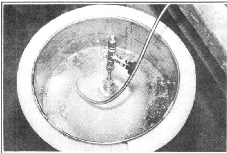
FIGURE B-13 About 30 Minutes Following Initial Dry Ice Introduction SCUBA Tank is at -80 Degrees Centigrade
