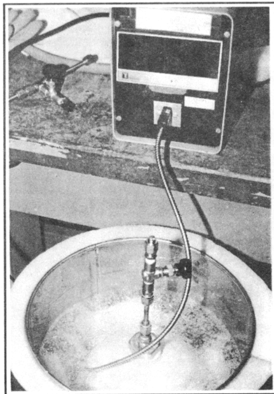
FIGURE B-11 15 Minutes After First Dry Ice Bricks Are Added A Temperature Probe Is Inserted
