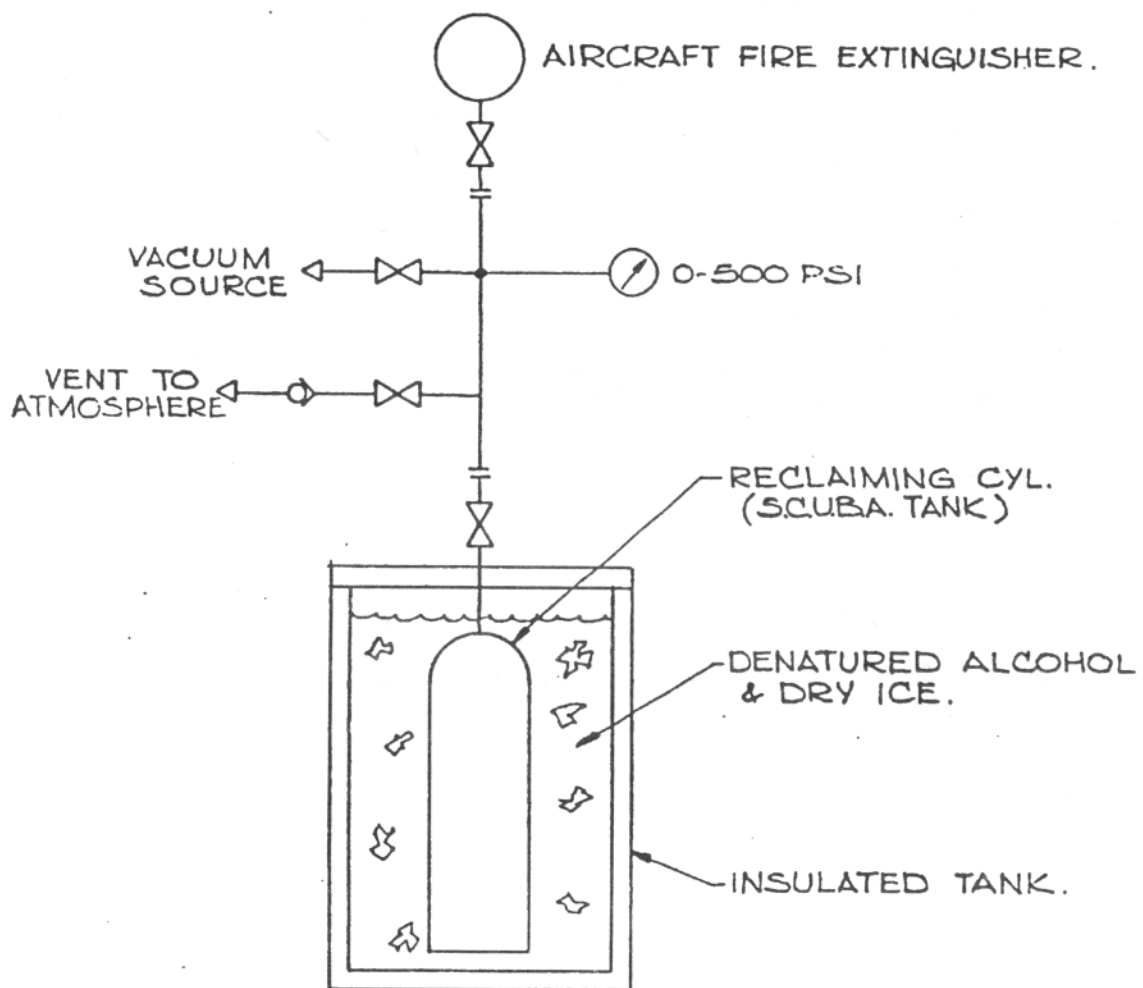
HALON RECOVERY SYSTEM
