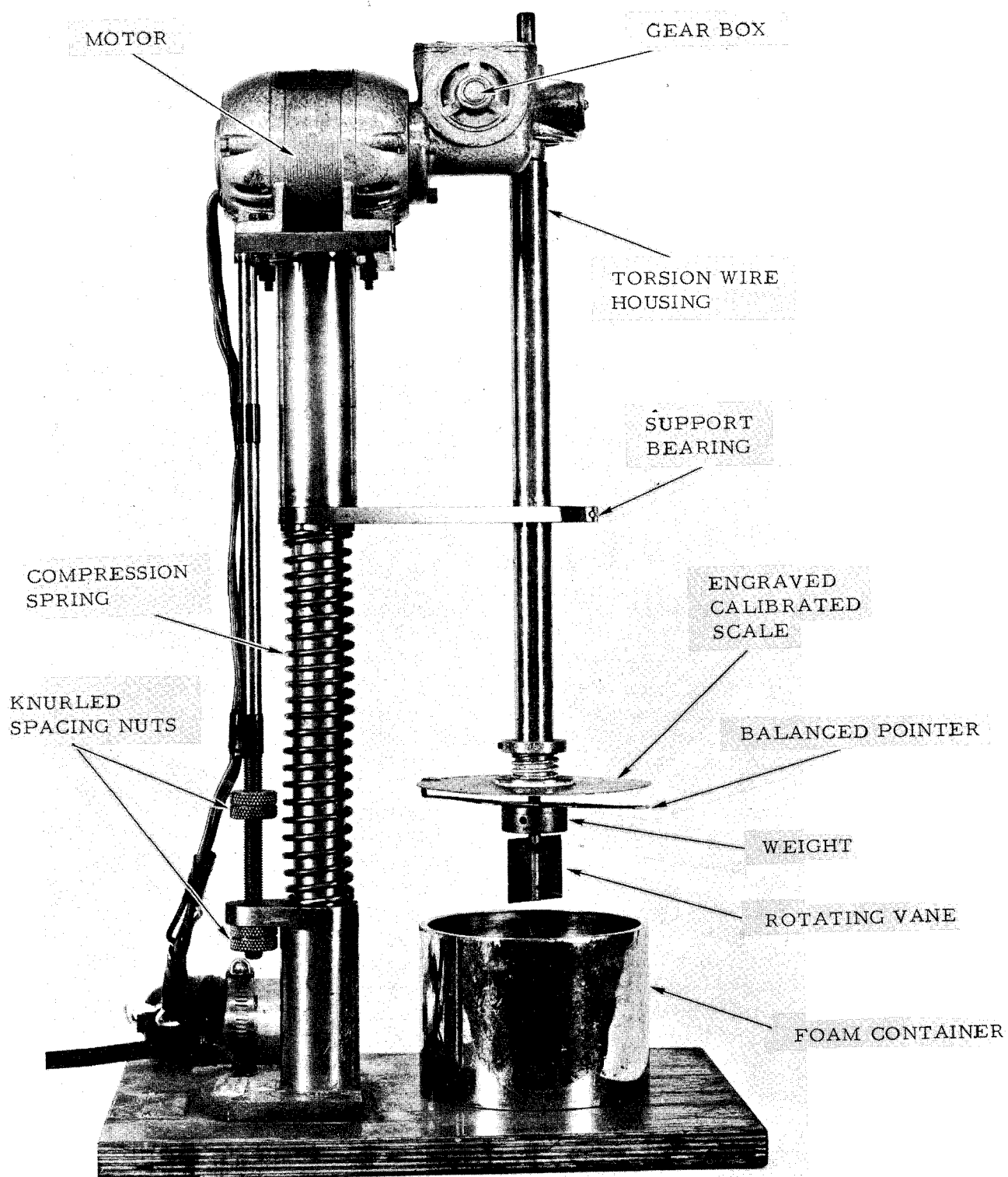
FIGURE 21 - FOAM VISCOMETER
