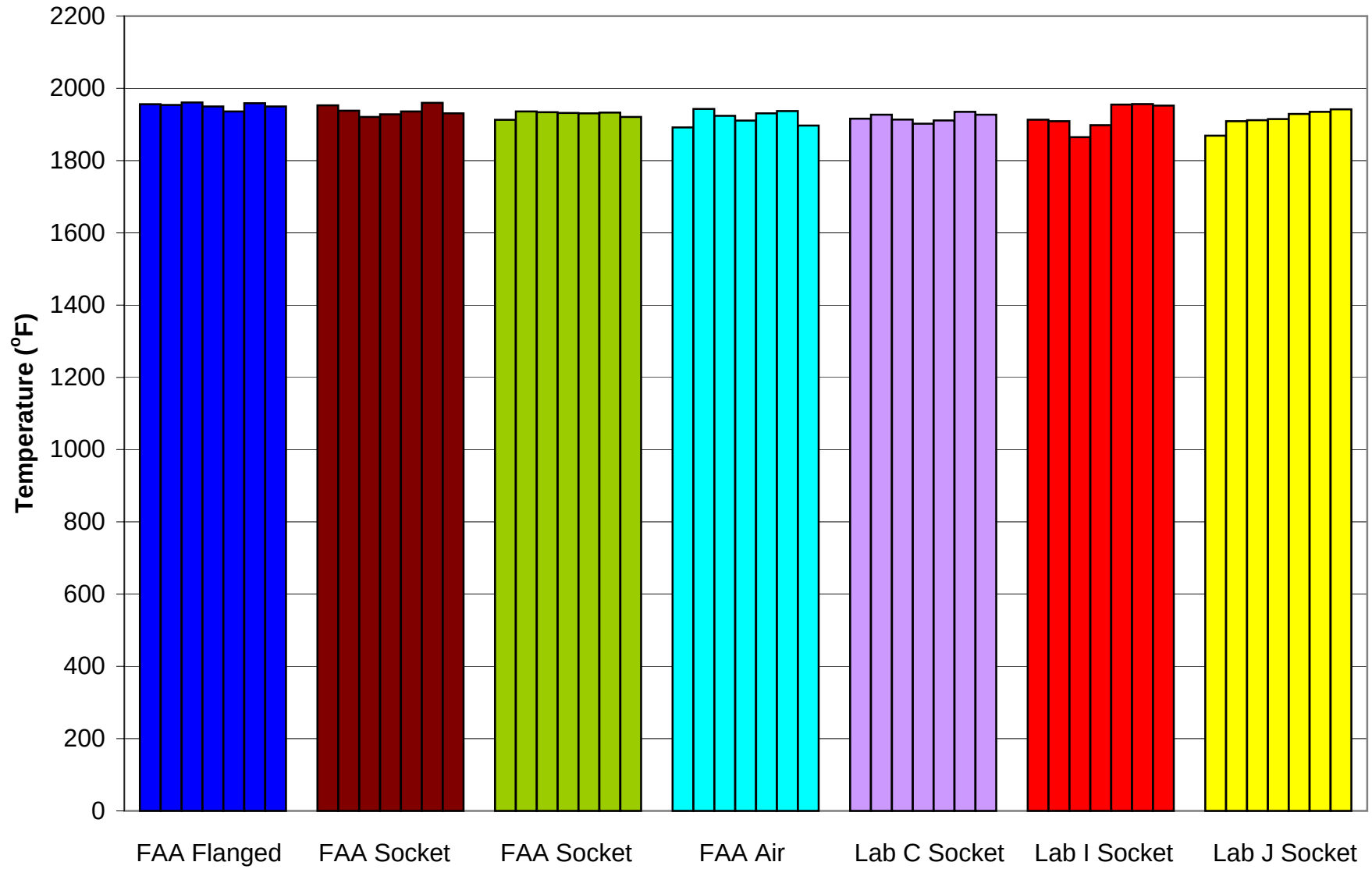
Initial Temperature Calibration
